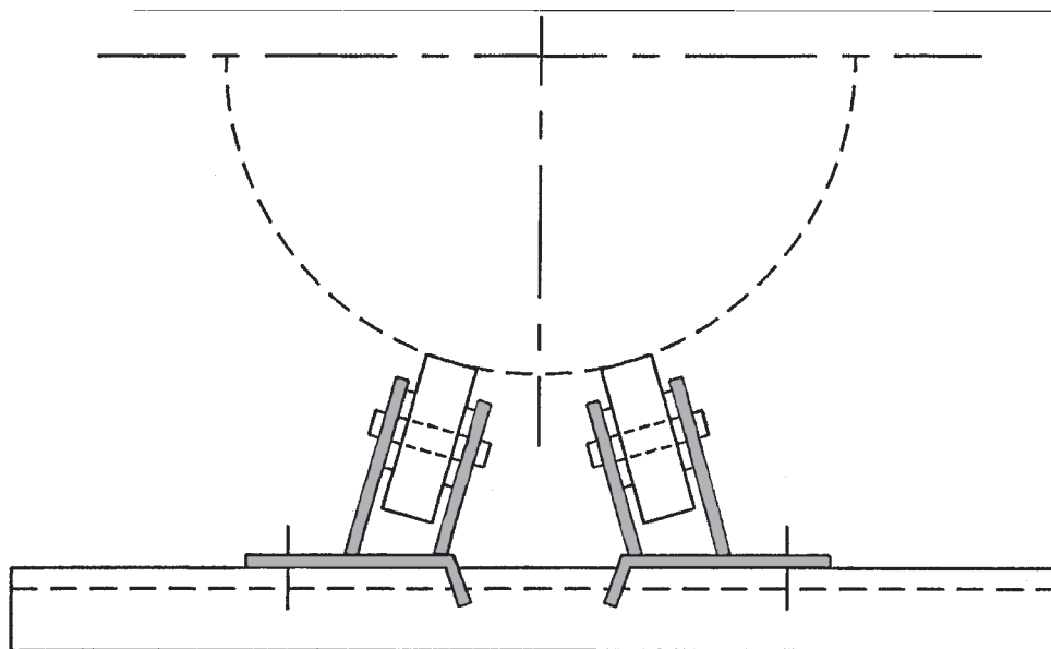
FM196 PIPE ROLLERS
