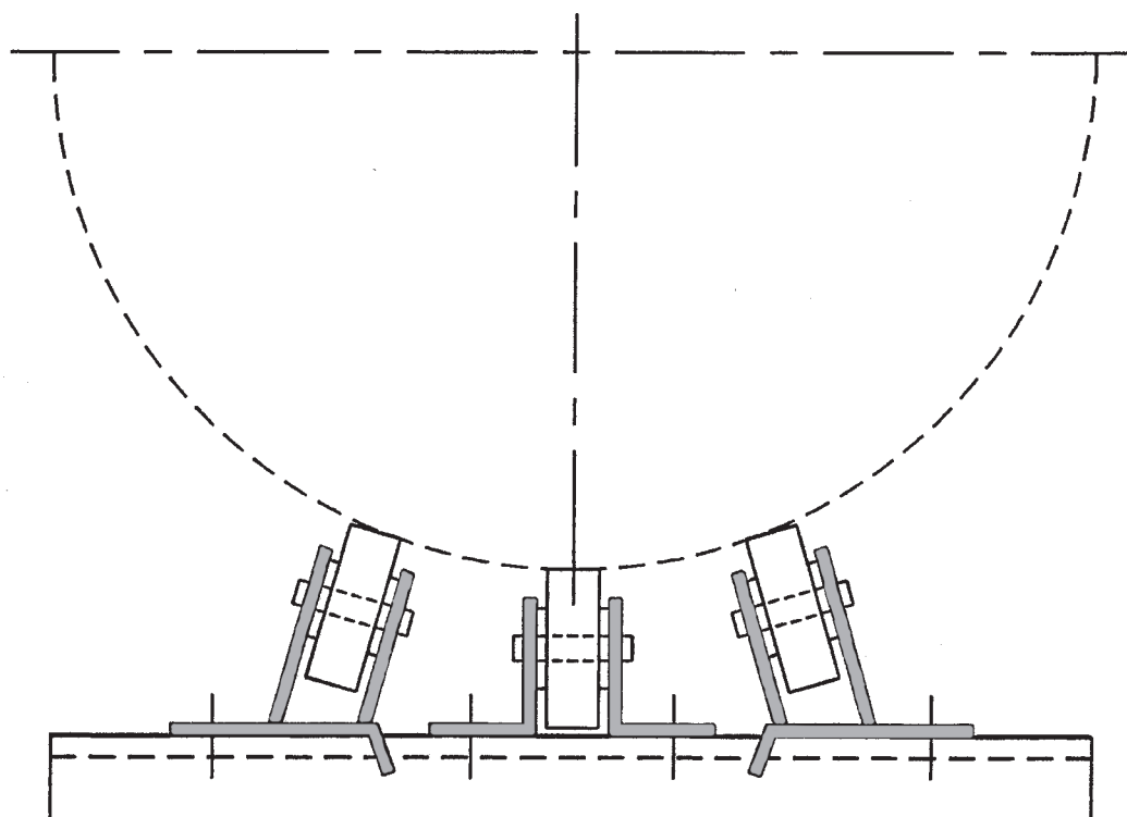
FM197 PIPE ROLLERS
